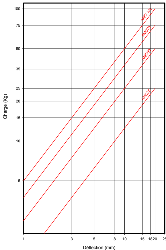
CHARGE DEFORMATION
